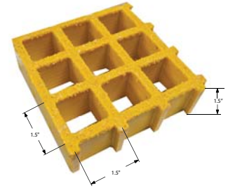
SQUARE MOLDED GRATING 3FT X 10FT SHEET WEIGHS - 123LBS 68% OPEN AREA
